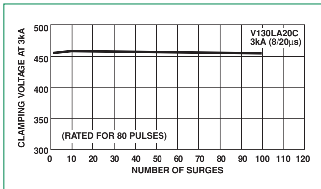
Figure 9. Typical Repetitive Surge Current Capability of C-III Series MOVs
