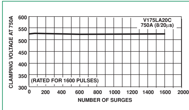
Figure 10. Typical Repetitive Surge Current Capability of C-III Series MOVs
