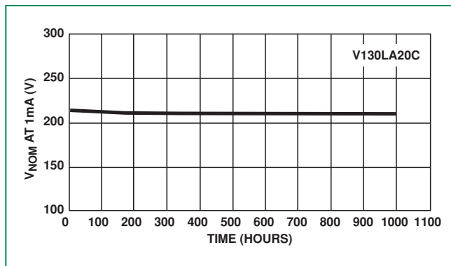
Figure 8. High Temperature Operating Life 125°C for 1000 Hours at Rated Bias
